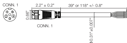
RB 5PIN STARTER CABLE 1M IP67 (AM400840055) RB 5PIN STARTER CABLE 3M IP67 (AM400850055)
