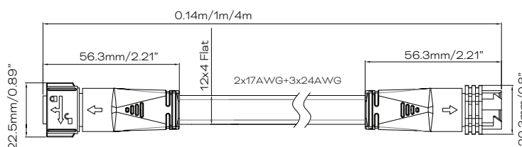
MT PRO INTER CABLE FLAT
