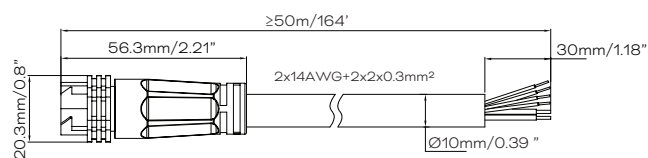
MT PRO STARTER CABLE 6-WIRE (≥50m/164') ROUND
