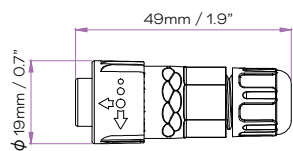
0-10V Starter Cable TYPE-2 DC 4-PIN (CE & ETL) (CA.SC.CCC01000 / CA.SC.CCC03000 / CA.SC.CCC05000 / CA.SC.CCC10000)
