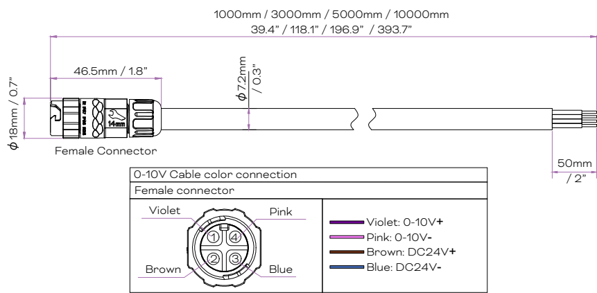
0-10V Starter Cable TYPE-2 DC 4-PIN (CE & ETL) (CA.SC.CCC01000 / CA.SC.CCC03000 / CA.SC.CCC05000 / CA.SC.CCC10000)
