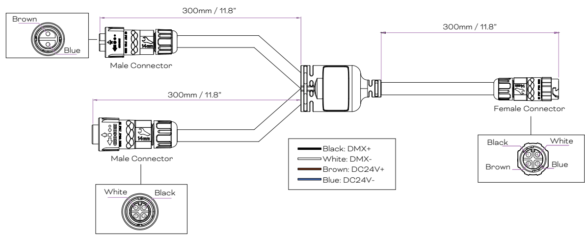
End Cap TYPE-2 DC 4/5-PIN With Terminator (CE & ETL) (CA.EC.CC100000)
